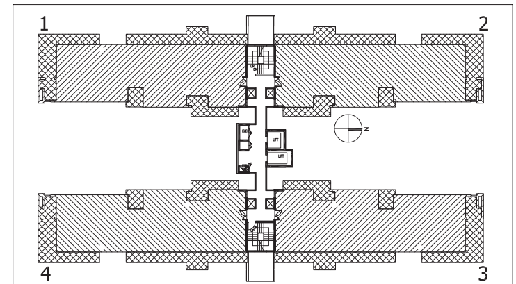
KEY PLAN OF FLOOR 6
