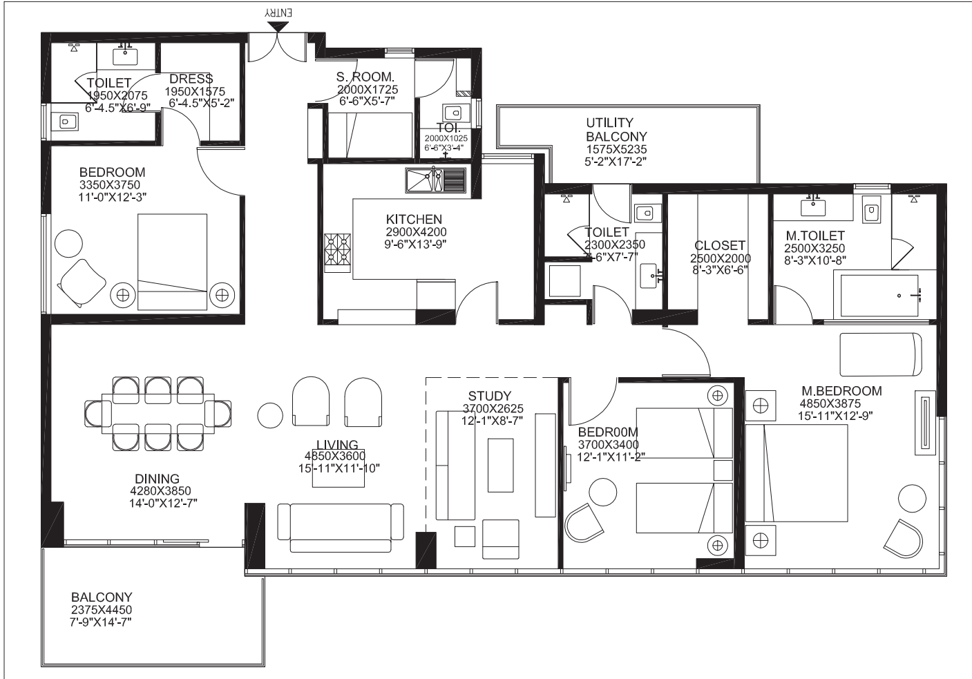
FLOOR PLAN
